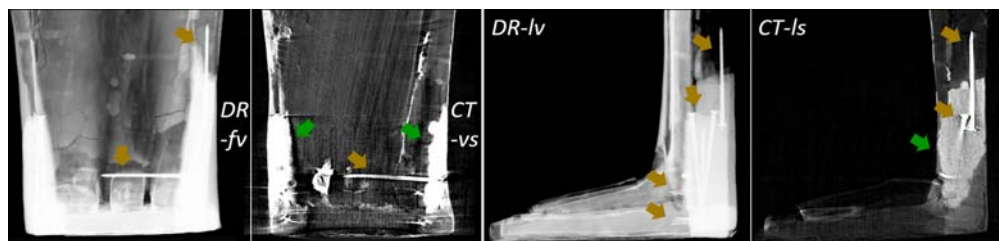
Fig. 7. Details of the feet of the coffin lid: a comparison between digital radiography (DR, both frontal view -fv- and lateral view -lv-) and significant sections from the computed tomography volume (CT, both vertical -vs-, and lateral -ls- sections) are shown. Coloured arrows indicate: material from previous restoration (dark green); modern screws (brown).
