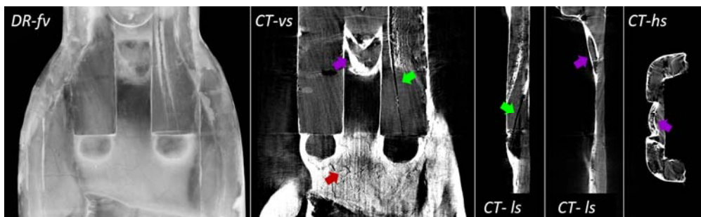
Fig. 4. Details of the upper part of the chest of the coffin lid: digital radiography (DR) and computed tomography (CT) vertical (vs), lateral (ls) and horizontal (hs) sections are shown. Coloured arrows indicate: crack in the wood (green); possible re-use (purple); cracks in the preparatory layer (dark red).
