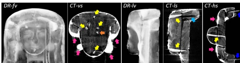
Fig. 3. Details of the head of the coffin lid: a comparison between digital radiography (DR, both frontal view -fv- and lateral view -lv-) and significant sections from the computed tomography volume (CT, both horizontal -hs-, vertical -vs-, and lateral -ls- sections) are shown. Coloured arrows indicate: wooden dowels (yellow); thick preparatory material layer (pink); filler material (orange); tenons and mortises (blue); an empty cylindrical hole (light blue).
