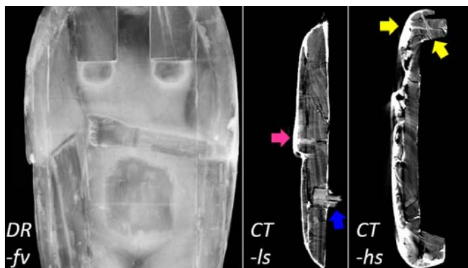
Fig. 5. Details of the arms and abdomen of the coffin lid: digital radiography (DR) and computed tomography (CT) lateral (ls) and horizontal (hs) sections are shown. Coloured arrows indicate: tenon and mortise (blue); thick preparatory material layer (pink); wooden dowels (yellow).
