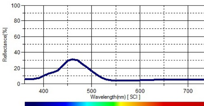
Fig. 3. Reflectance spectra of phtalocyanine blue (PB 15).
