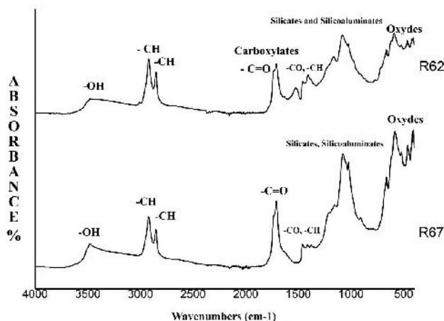
Fig.6. FT-IR spectrum of sample R67, collected from a ceramic pot used by Mariano in paint manufacture (below) and FT-IR spectrum of sample R62, collected from a paint tube probably filled by Mariano himself
