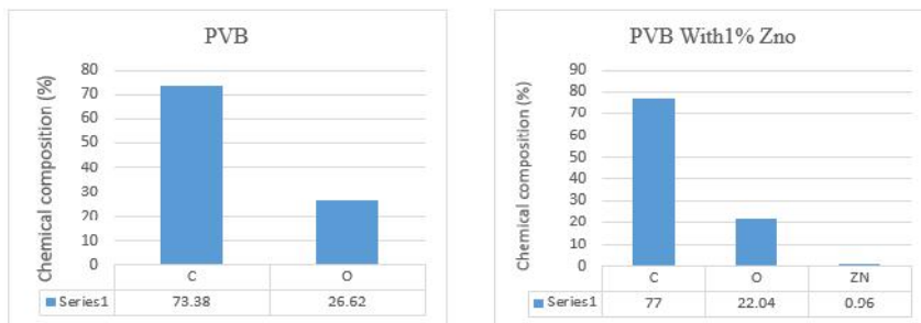
Fig. 5. Chemical composition (%) of samples treated with PVB (a); samples treated with PVB with nano-ZnO (b).
