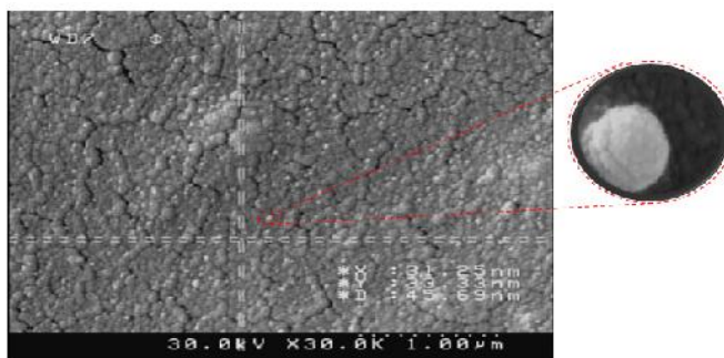
Fig. 6. FESEM micrographs of cross section, consolidated pieces by total immersion in PVB solutions with nano-ZnO additives in 1.0% ZnO
