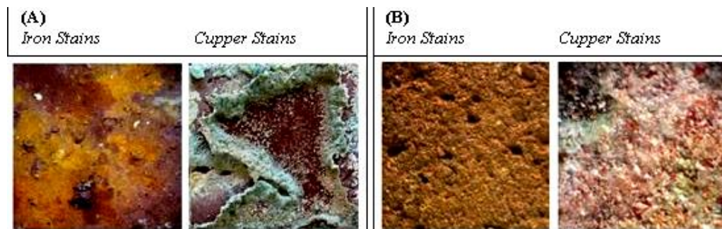
Fig. 3. OLS photos of brick samples a. iron corrosion layers & copper stains before cleaning, b. the same samples after plasma cleaning
