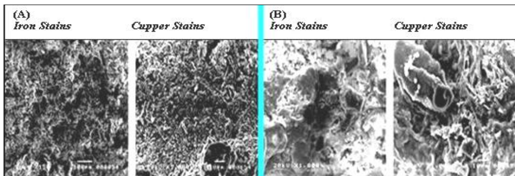
Fig. (4) SEM photomicrographs of brick samples a iron corrosion layers & copper stains before cleaning, b the same samples after plasma cleaning
