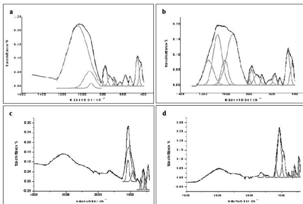
Fig. 5. FTIR spectrum of brick surface a with iron corrosion layers, b after plasma cleaning c with copper stains, d after plasma cleaning
