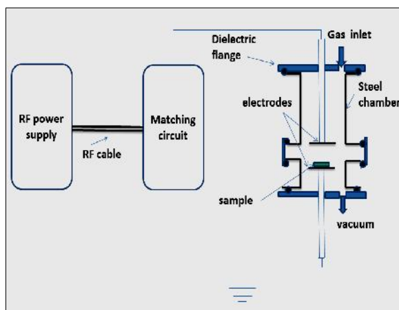
Fig. 2. Schematic diagram of the CCP cleaning experiment arrangement
