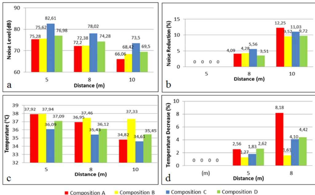
Fig. 3. Graphics of values for each vegetation composition: a - Average of Noise Level, b - Average of Noise Reduction, c - Average of Temperature, d - Average of Temperature Decrease
